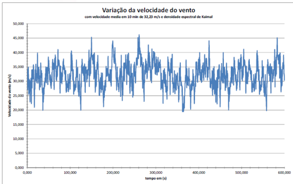
Figure 5. Wind Velocities Variation in m/s.
