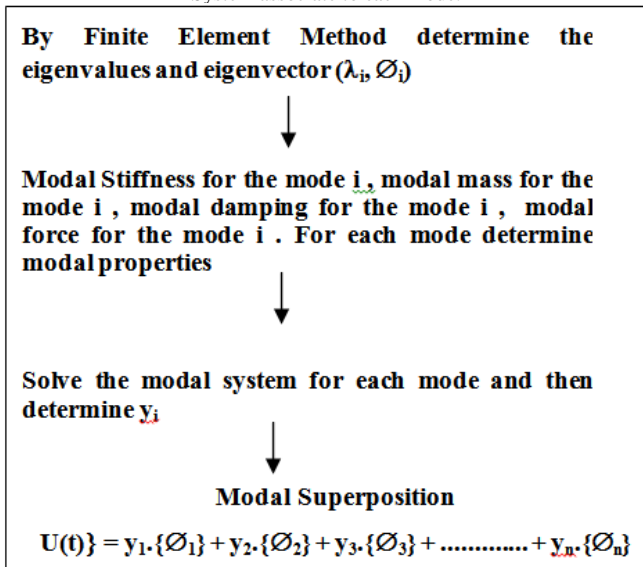
Figure 3. General steps for Modal Superposition to obtain the Response Structural Dynamics of the Tower.
