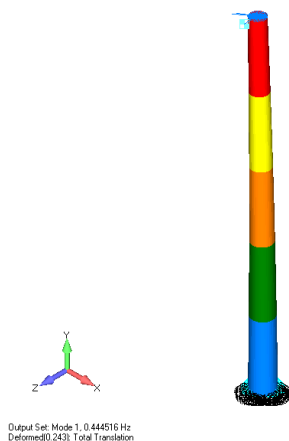
Figure 9. Thin Shell Element Model – First Natural Mode of Vibration. First Mode Natural frequency is 0.44 Hz. Both models have the same natural frequency.
