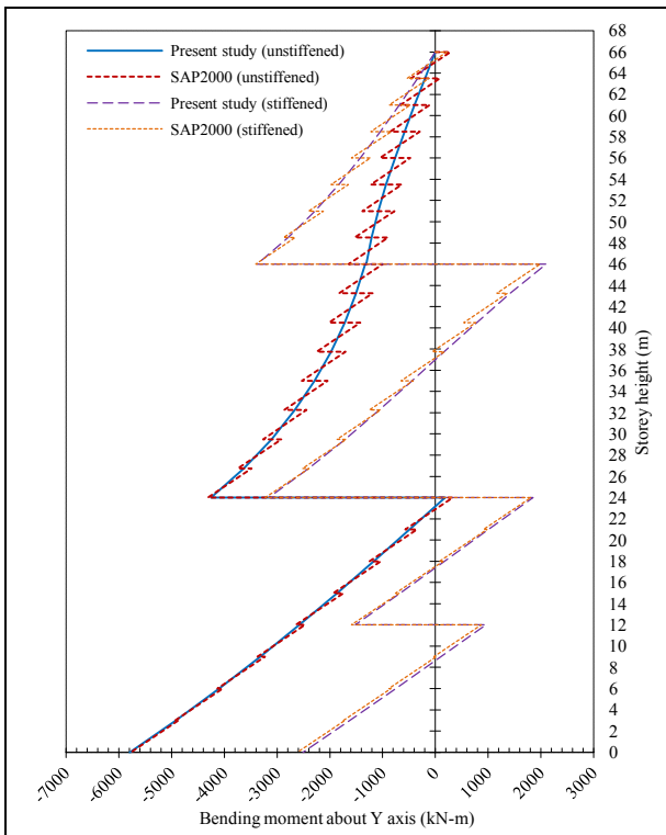
Figure 5. The total shear wall bending moment about Y axis along the height.
