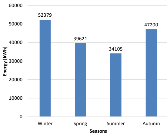
Figure 4. Seasonal total energy requirement of LED and driver.
