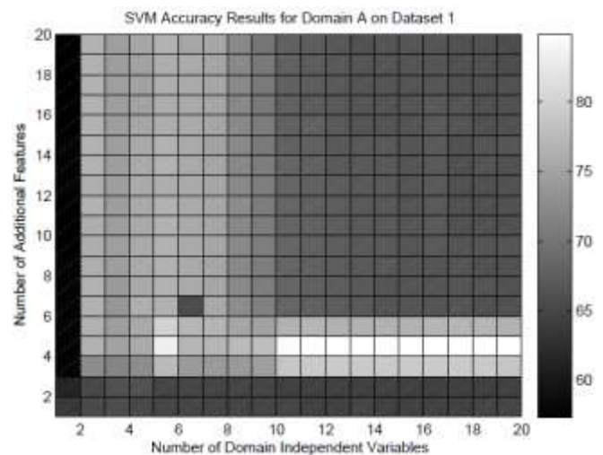
Figure 11. SVM Accuracy Results for Domain A on Dataset 1 after SFA
