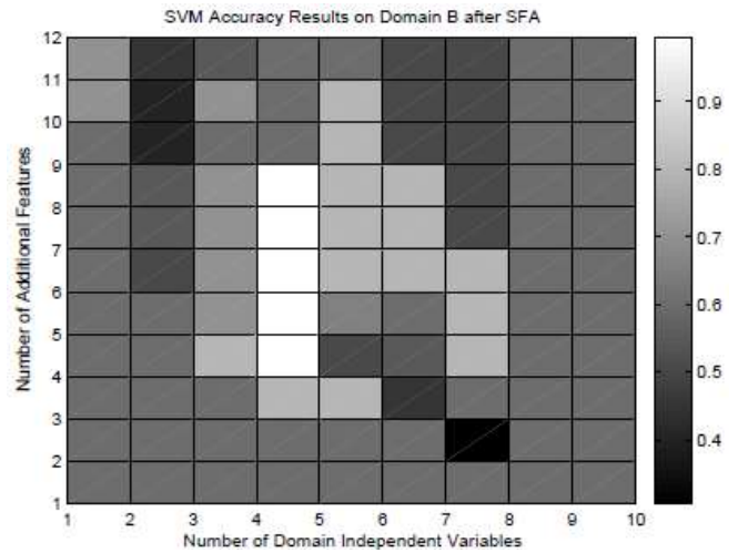
Figure 8. SVM Accuracy Results on Domain B after SFA
