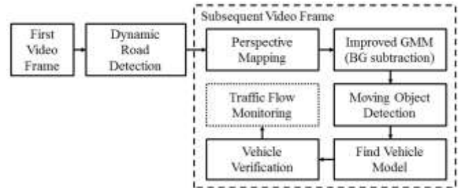
Figure 1. Proposed vehicle detection system.
