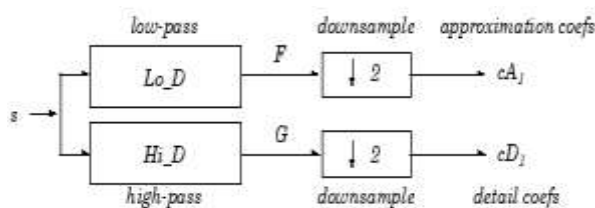
Figure 8: MWT decomposition structure
