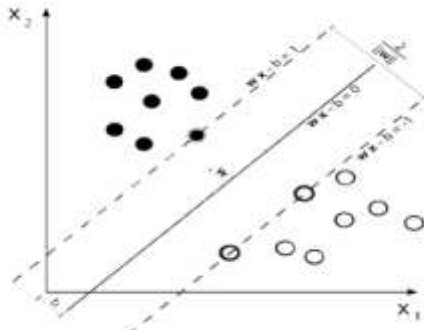
Figure 9: Working of SVM
