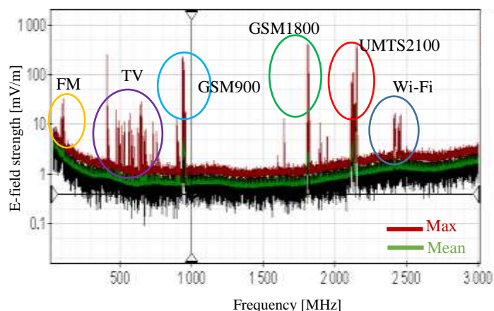
Figure 4. Detailed examination of the signal in the frequency domain between 100 kHz-3 GHz
