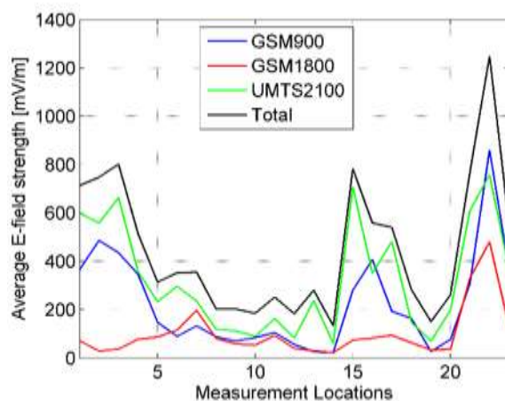
Figure 8. Band selective EMR measurements in the Campus
