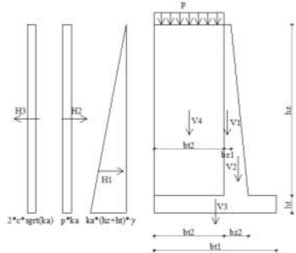
Figure 1. Retaining wall
