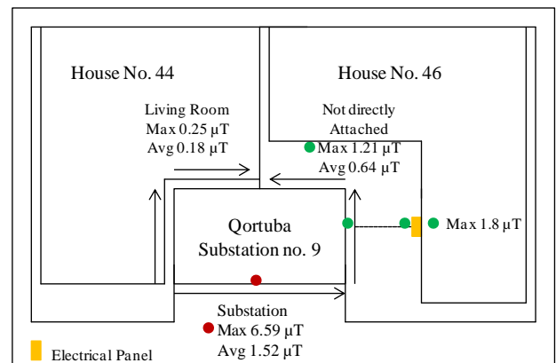
Figure 5. A schematic diagram presenting magnetic field levels in the vicinity of substation No.9
