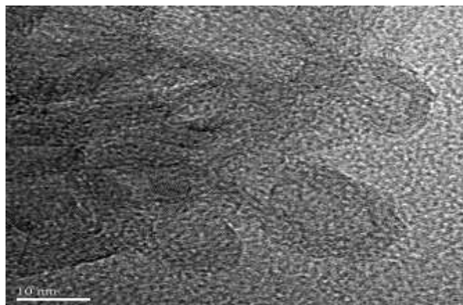
Fig. 2. TEM image for the catalytic detonation of TNT to synthesis various nanocapsules using Ti catalyst.
