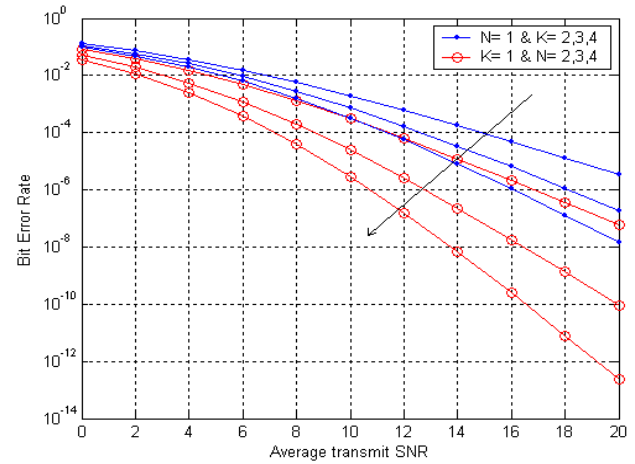
Figure 2. Comparing the BER performance as a function of transmit SNR with increasing the number of antennas and relays by turn when \bar{\gamma}_1 = \bar{\gamma}_2 = 1.5 & \bar{\gamma}_o = 3 .
