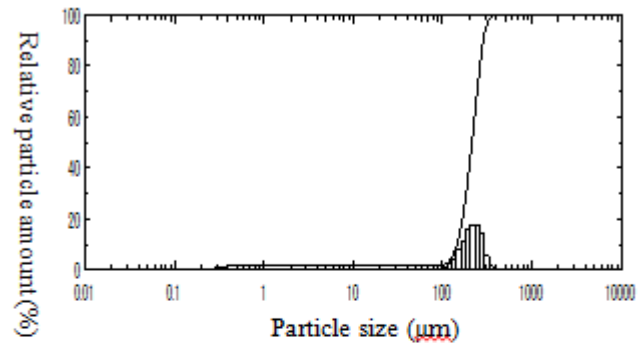
Figure 2 Particle size distribution of slag
