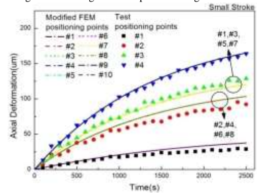
Fig. 10 Positioning error comparison in small stroke case
