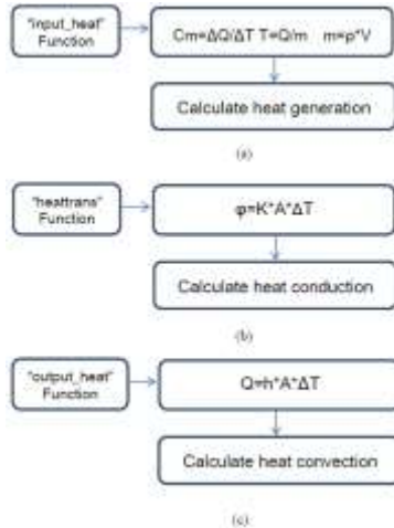
Fig. 5 Formula of computational process of Function
