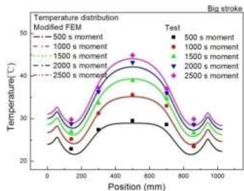
Fig. 12 Temperature distribution in big stroke case
