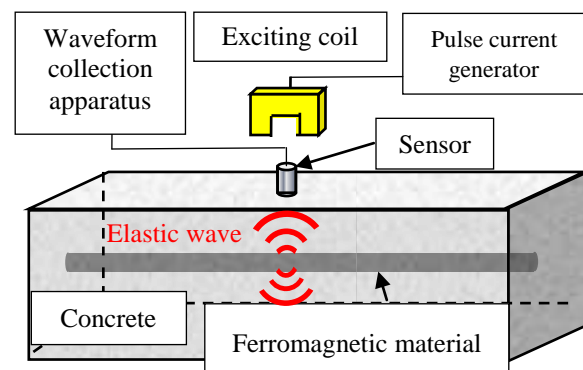
Figure 1. Outline of electromagnetic pulse method.
