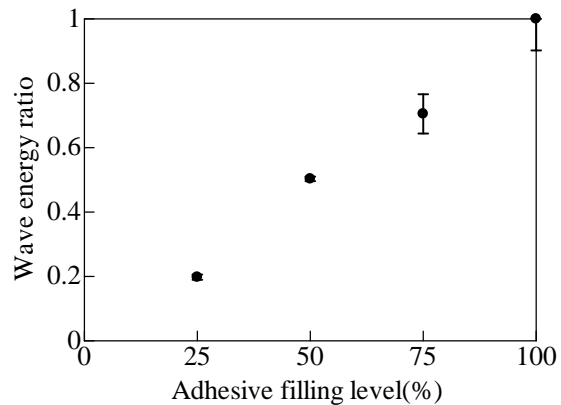
Figure 9. Relationship between wave energy ratio and adhesive filling level (with permanent magnet).
