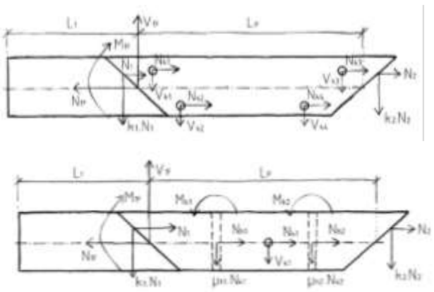
Figure 3. Distribution of forces in a four-dowel joint with oblique faces (top) and joint with two vertical wooden pegs and one dowel (bottom)
