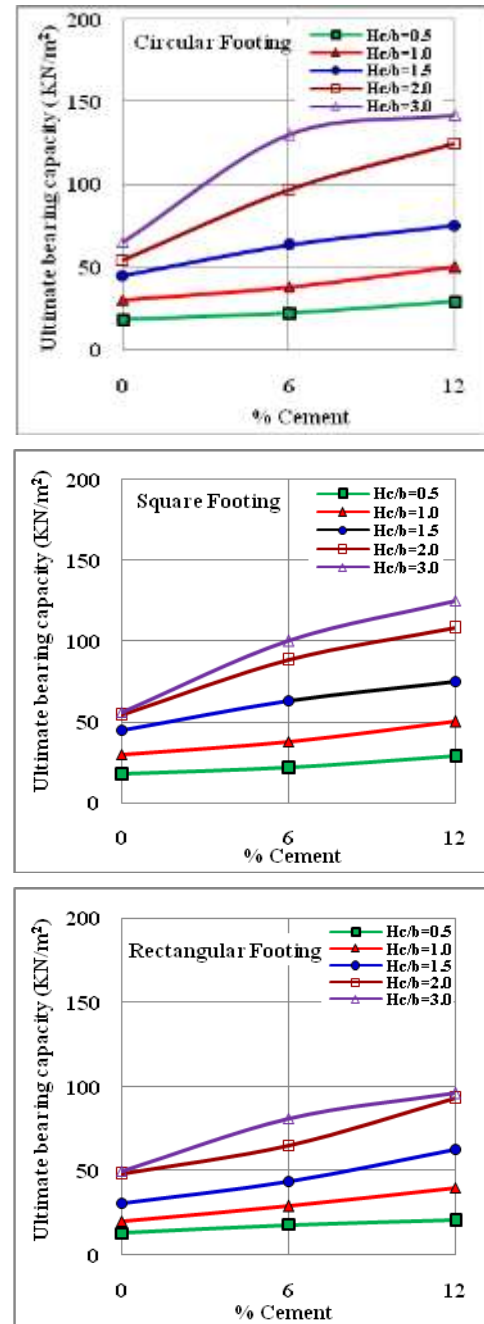
Figure 8. Effect of cement % on bearing capacity with tickness of sand layerk, Hc/b ratio.
