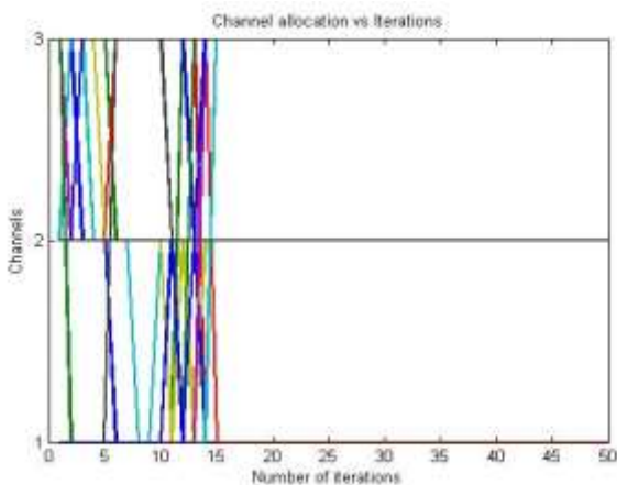
Fig. 4: Channel convergence
