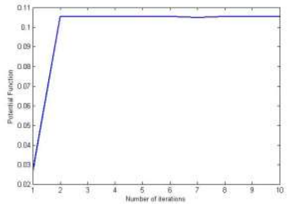
Fig. 3: Potential Function
