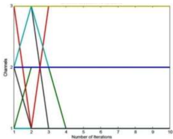
Fig. 2: Channel Convergence
