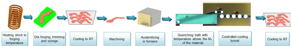
Figure 6. Manufacturing route for forged parts involving heat treating with Q&P process and direct cooling in bath
