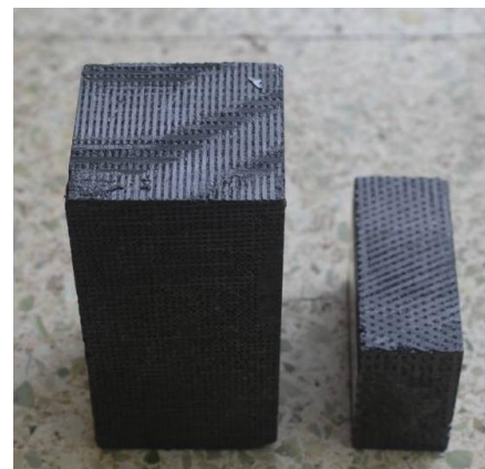
Fig: 10. 3-D and 4-D Carbon-Carbon densified blocks
