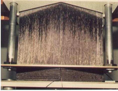
Fig: 6 Shows the dry weaving process
