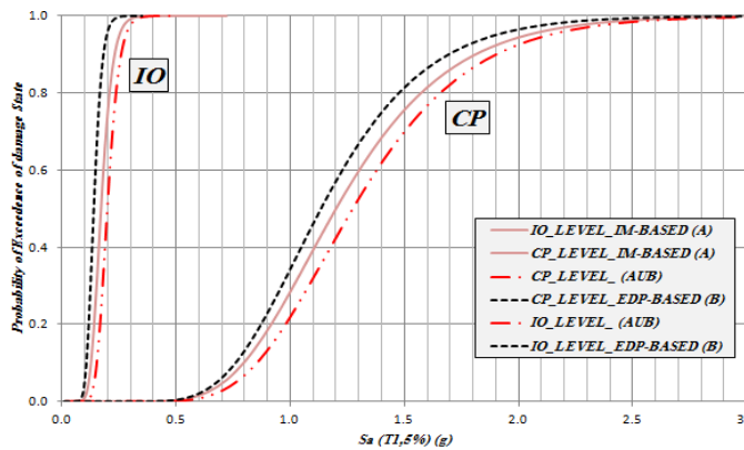
Figure 6. Derived fragility curves for IM-Based approach (P(A)) And EDP-Based approach (P(B)) and combination of them; at two levels of IO & CP damage states, for frames with low-ductility.
