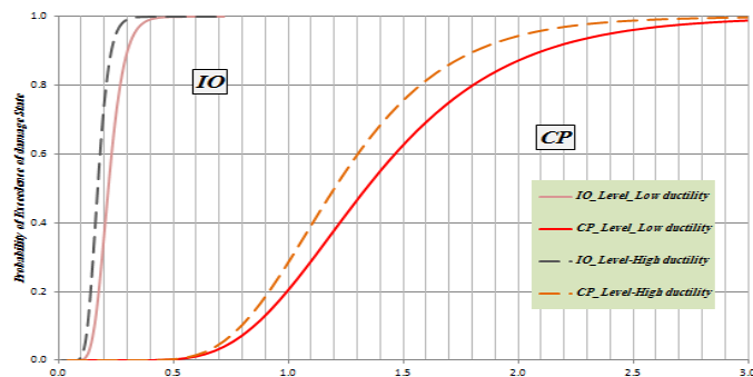
Figure 8. IM-Based fragility curves at two levels of IO & CP damage states; for frames with low & high-ductility.
