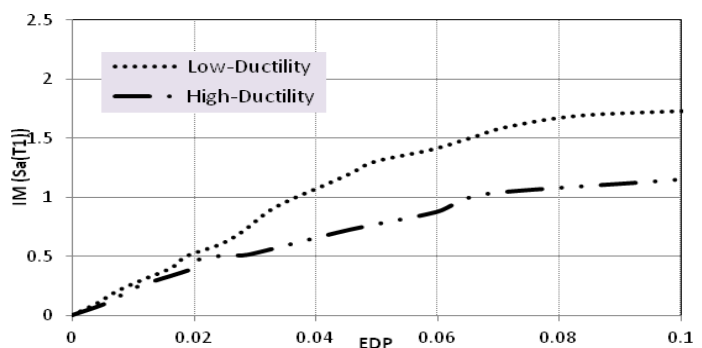
Figure 3. Comparison of median IDA curves for low & high ductile frames.
