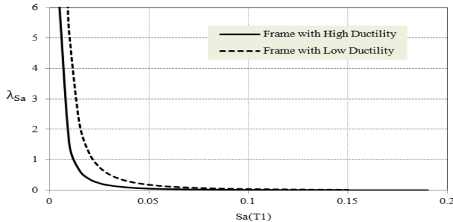
Figure 10. Seismic hazard curve for understudied structures; in high hazard region.
