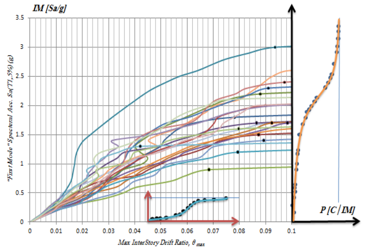
Figure 4. EDP-Based approach for derivation of fragility curves; for IDA curves in Fig. 2.
