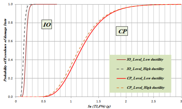
Figure 9. EDP-Based fragility curves at two levels of IO & CP damage states; for frames with low & high-ductility.
