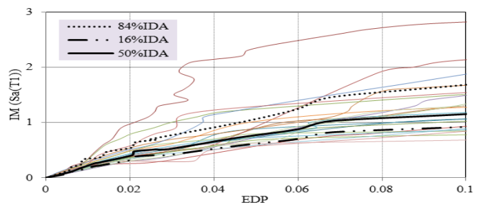
Figure 1. Obtained IDA curves for high-ductile frame
