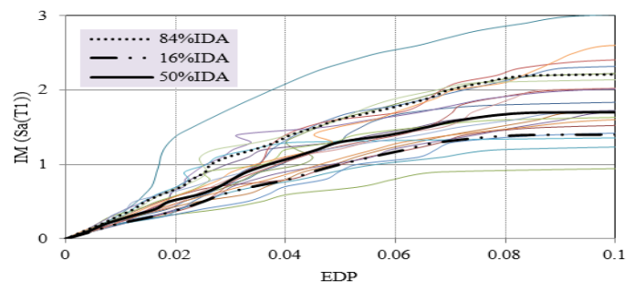
Figure 2. Obtained IDA curves for low-ductile frame.
