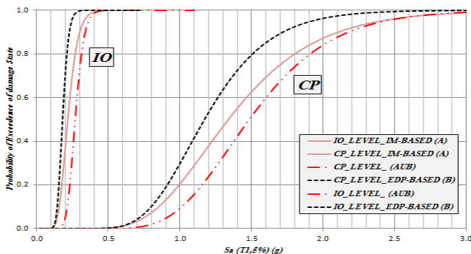
Figure 7. Derived fragility curves for IM-Based approach (P(A)) And EDP-Based approach (P(B)) and combination of them; at two levels of IO & CP damage states, for frames with high-ductil.
