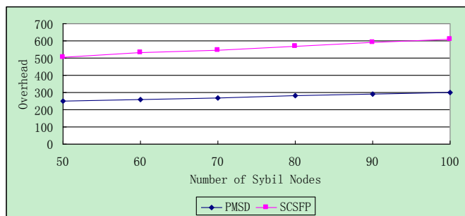
Figure. 5 Total overhead
