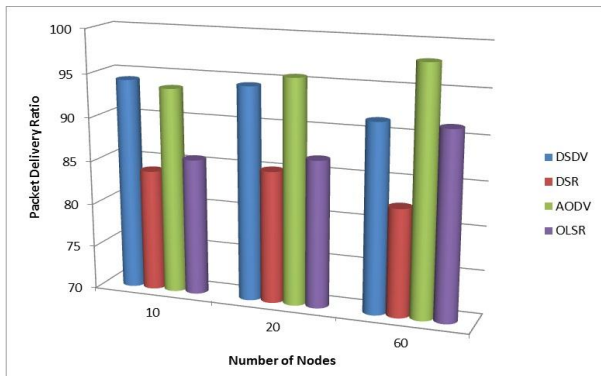
Figure3. Packet Delivery Ratio for AODV, DSR, DSDV and OLSR
