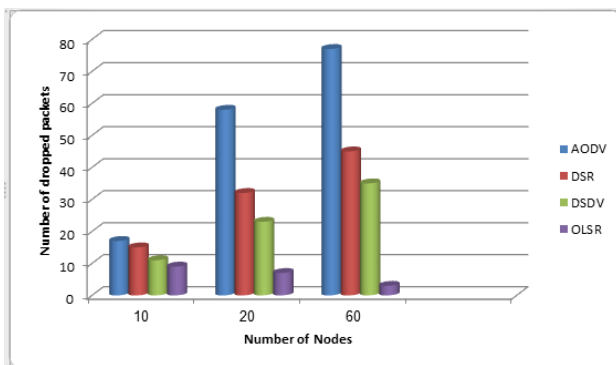
Figure6. Number of Dropped packets for AODV, DSR, DSDV and OLSR
