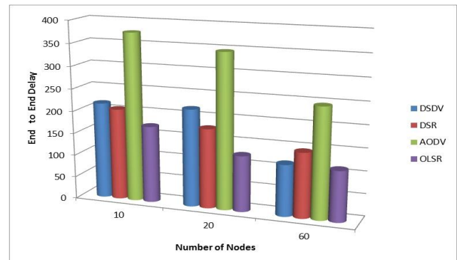
Figure5. End-to-End delay for AODV, DSR, DSDV and OLSR
