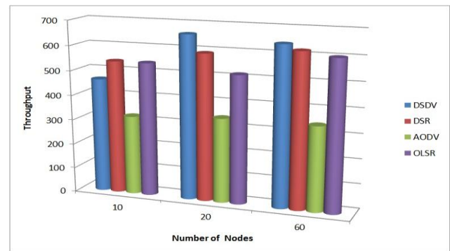
Figure4. Throughput for AODV, DSR, DSDV and OLSR
