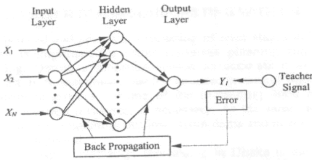
Figure 2. Layers of ANN
