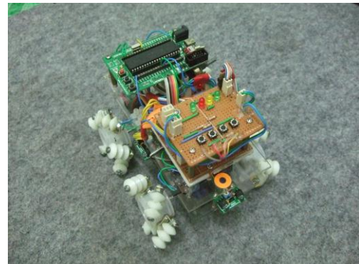
Figure 3. Multi-Movement Mobile Robot using Mecanum Wheels
