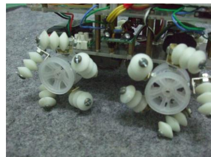
Figure 4. Mecanum Wheels using Abacus Beads
