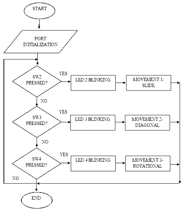
Figure 6. Flowchart for special movement mode
