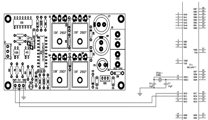
Fig 5 Driving motor board connected to microcontroller
