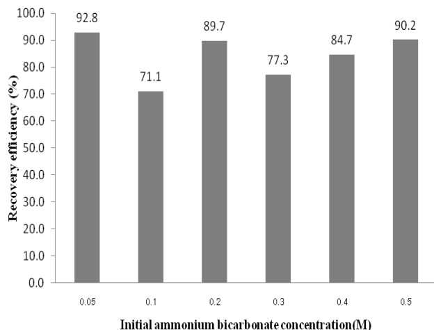
Figure 3. Ammonia and carbon dioxide gas recovery efficiency
