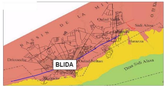
Figure 4. Water network and ground conditions
