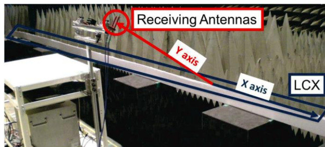
Figure 4. View in the anechoic chamber
