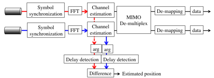
Figure 8. Receiver configuration[12].
