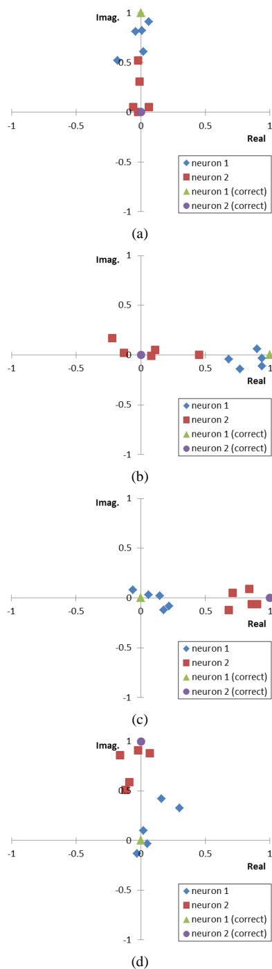
Figure.5 Output results for each motion input; (a) extension, (b) flexion, (c) grasp, and (d) open.
