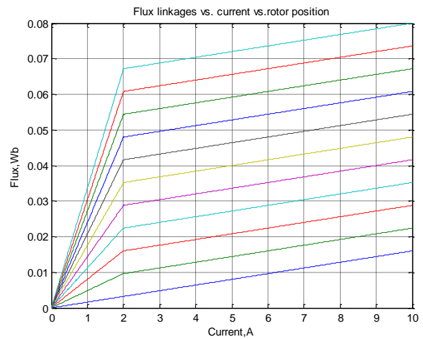
Figure (2) flux linkage vs current vs rotor position
