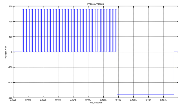
Figure (12) Phase A voltage (zoomed)
