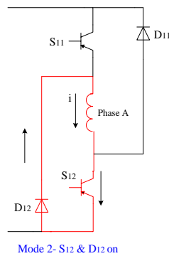
Figure (1.1) Half-bridge first mode (Fluxing)
