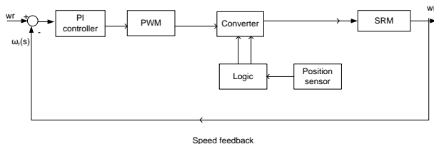
Figure (5) SRM basic control structure
