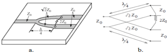
Figure 11. a. An equal-split WPD in microstrip form; b. Equivalent transmission line circuit.
