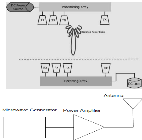
Figure 1. The block diagram of transmitter unit of Wireless power transmission system.
