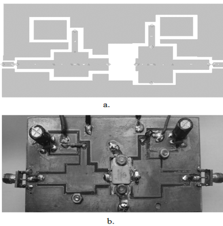
Figure 6. a. Layout of the power amplifier; b. The fabrication of the amplifier.
