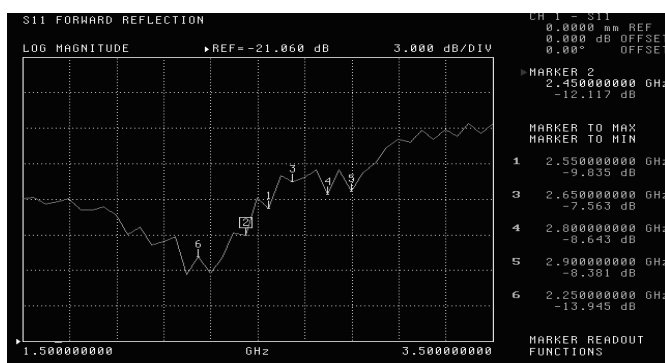
Figure 16. The value of S11 on the Network Analyzer.
