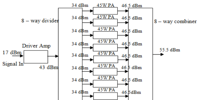
Figure 2. Block diagram of the proposed SSPA.
