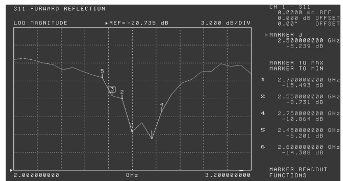
Figure 9. The value of S11.
