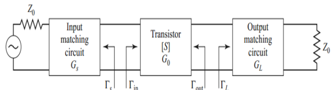
Figure 4. The general transistor amplifier circuit.
