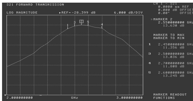
Figure 7. The amplitude of S21 in dB of the amplifier.
