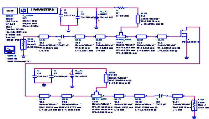
Figure 5. Schematic of the power amplifier.
