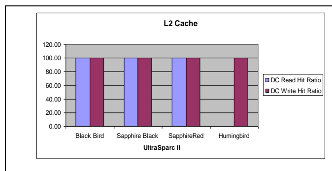
Figure 6. Graphical result of L2 Data Cache
