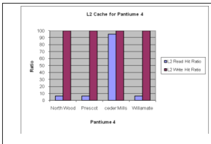
Figure 2. Graphical result of LI Data Cache
