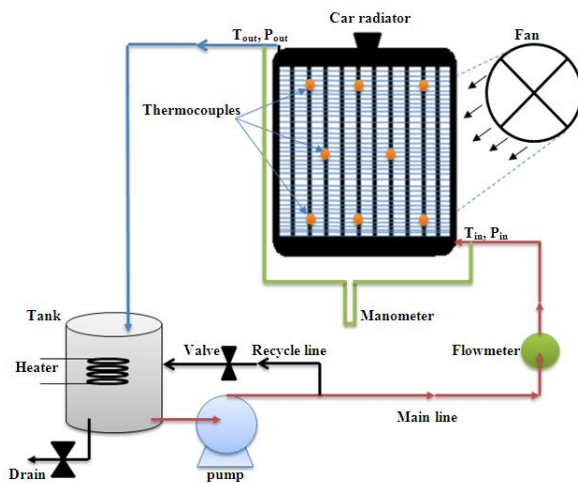
Fig. 1. Schematic diagram of test rig
