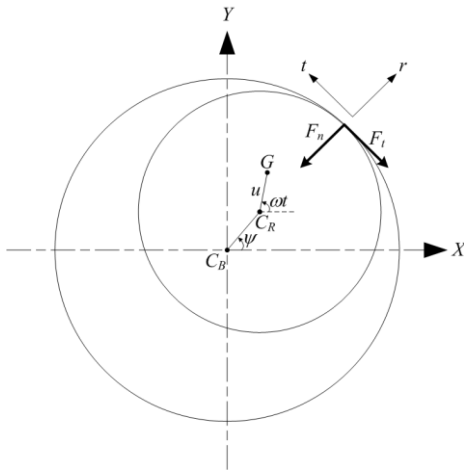
Fig. 1. Rotor-to-stator contact model
