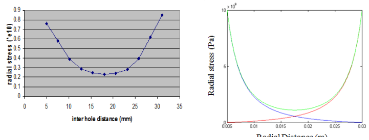
Figure 7 a. Variation of normal stress along the radial direction for C/D = 3.6 & 4% expansion
