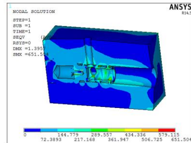
Fig 6: Result for Check Valve at pressure of 48.26Mpa and Temperature at 71.1 o C
