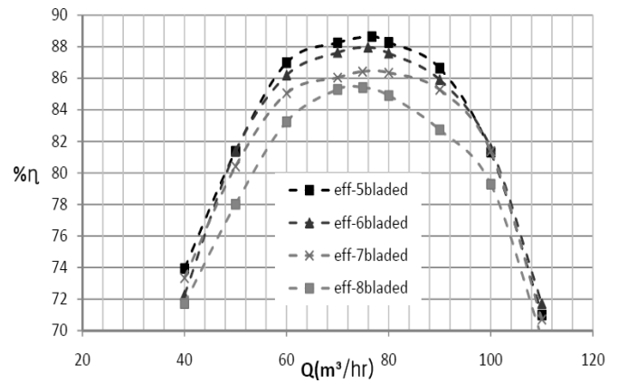
Figure 5. Efficiency curves of different bladed impellers
