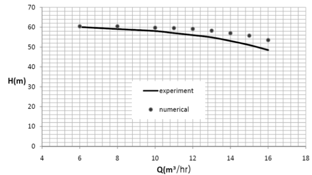
Figure 2. Comparison of numerical and experimental head-capacity curves
