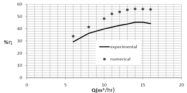
Figure 3. Comparison of numerical and experimental efficiency curves
