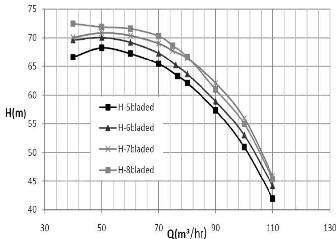
Figure 4. Head-capacity curves of different bladed impellers
