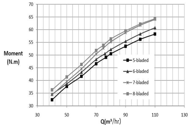
Figure 6. Moment needed of different bladed impellers at constant rotational velocity of 2900rpm
