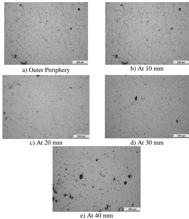
Figure 3. Optical microstructures of AA 6061 centrifugal cast ring taken at different locations starting from outer periphery towards inner periphery
