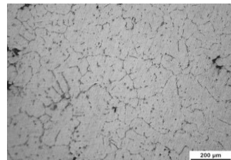
Figure 2. AA 6061 Gravity Microstructure
