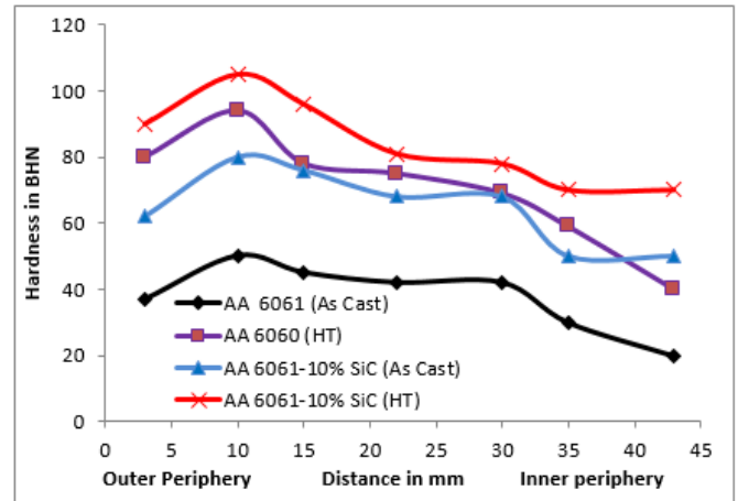
Figure 6. Brinell hardness of AA 6061 – 10% SiC FGMMC rings from outer to inner periphery, both in as cast and T6 heat treated condition
