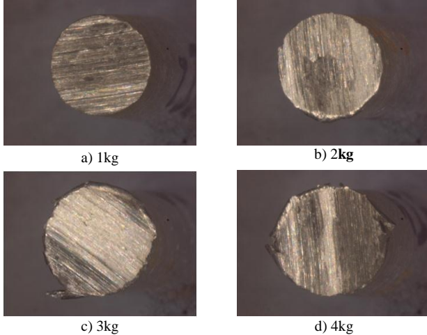
D) AA 6061-10% SiC FGMMC inner pin: wear surfaces at different loads
