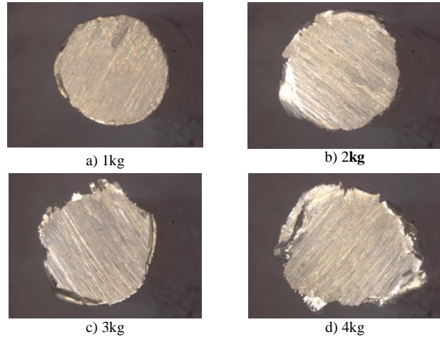
A) AA 6061 outer pin: wear surfaces at different loads
