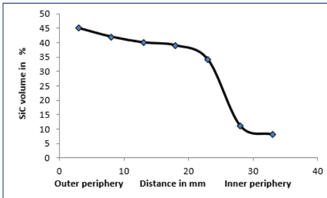
Figure 5. Volume percentage of silicon carbide in AA 6061 – 10% SiC FGMMC ring from outer periphery towards inner periphery of the casting.
