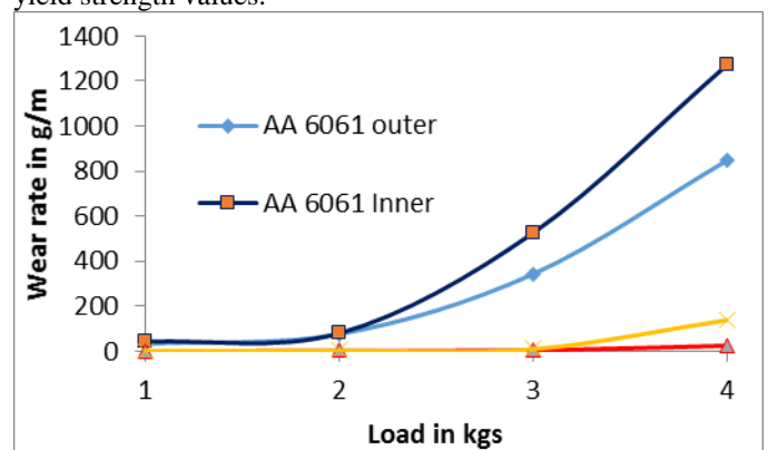
Figure 7. Pin on disc wear rate of AA 6061 and AA 6061-10% SiC FGMMC pins of inner and outer zones.
