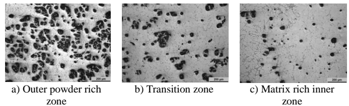
Figure 4. Optical micrograph of AA 6061–10% SiC FGMMC ring taken at different regions starting from outer periphery towards inner periphery
