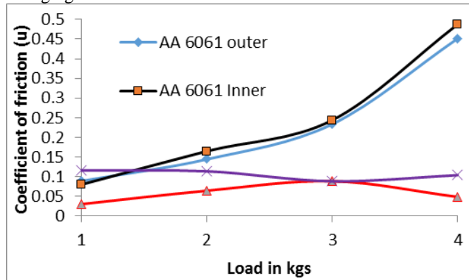
Figure 8. Pin on disc coefficient of friction of AA 6061 and AA 6061-10% SiC FGMMC inner and outer pins.
