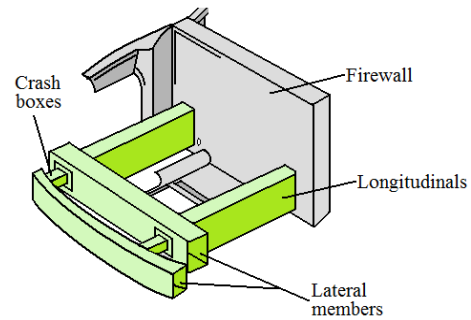
Figure 2: Crash box location in frontal longitudinal
