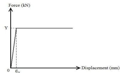
Figure 1b: An ideal force-displacement
