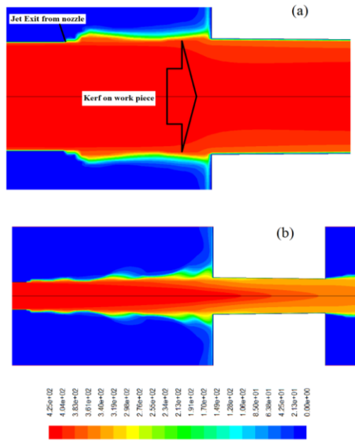
Fig 8. Countour plot of jet velocity distribution on workpiece
