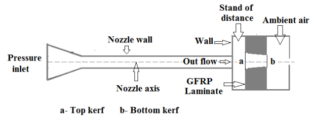
Fig.1. Computational model of AWJ Machining process
