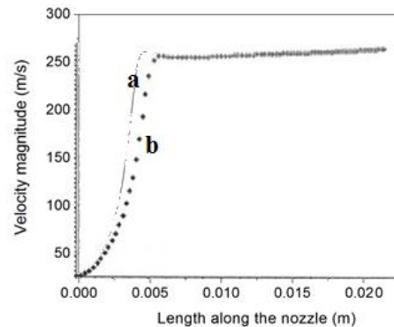
Fig. 3. The velocity distribution : a- velocity profile reproduced in the present work as against the velocity profile obtained by Gua et al
