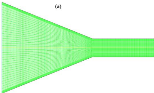
Fig. 2 A portion of the meshed domain near the critical section of AWJ nozzle
