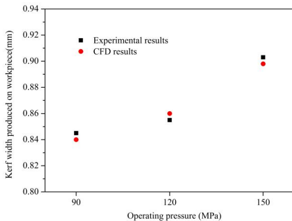
Fig 5. The kerf width on workpiece at various pressures
