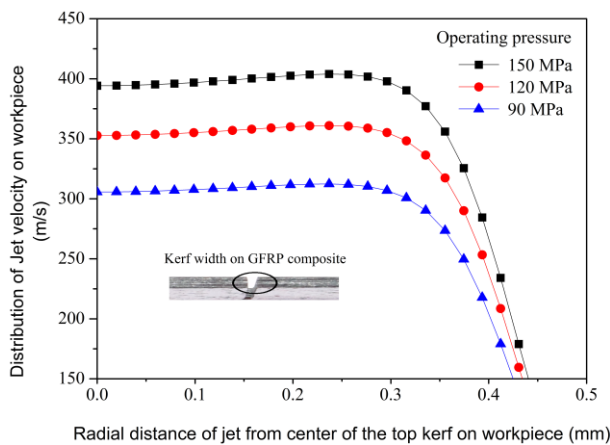
Fig 4. Plot of jet velocity distribution on workpiece at various pressures
