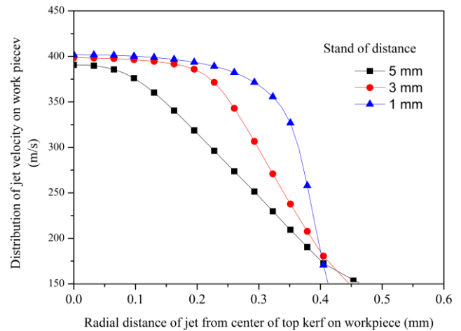
Fig 6. Plot of jet velocity distribution on workpiece at various SOD
