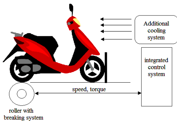
Fig.1: Layout of basic chasis dynamometer for a two wheeler under test. A control system has a hold over the speed and torque
