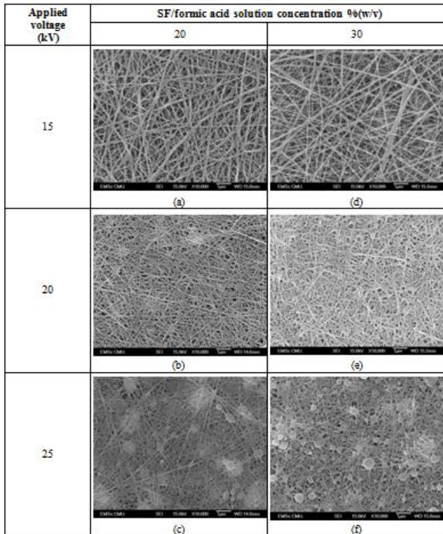
Figure 2. FESEM images of electrospun SF-nanofibers and their corresponding processing parameters of electric field of 15, 20 and 25 kV and concentrations of 20 and 30% (w/v), respectively.
