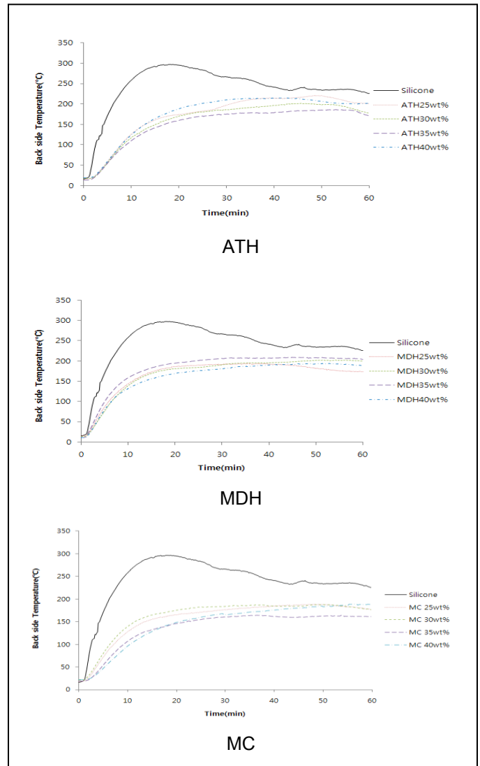
Fig. 6 Result graphs on the test of flame resistance
