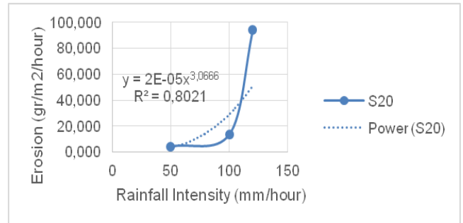
Figure 6. Regression graph of soil erosion with rainfall intensity for the slope of 20°
