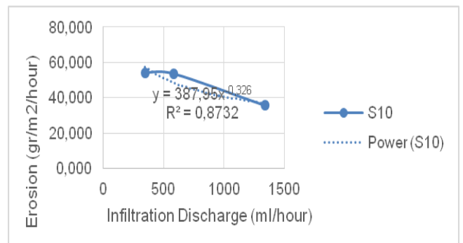
Figure 8. Regression graph of soil erosion with infiltration discharge for the slope of 10°
