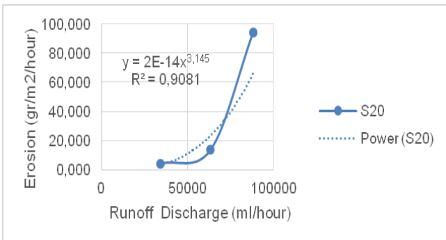
Figure 3. Regression graph of soil erosion with runoff discharge for the slope of 20°
