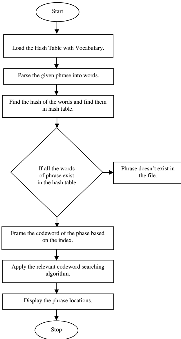
Figure 2. Flow chart for codeword searching
