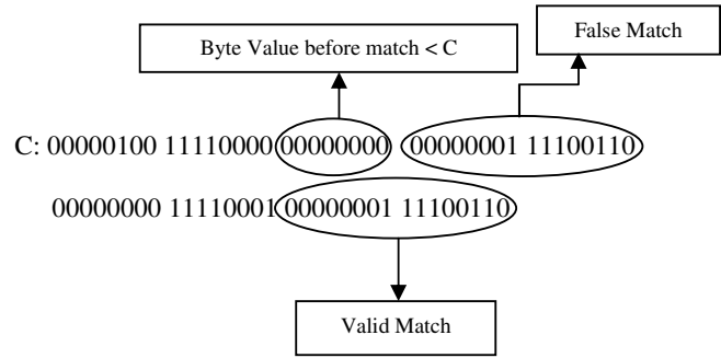
Figure 1. Pattern matching in compressed file.
