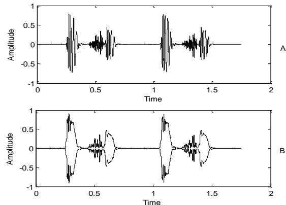
Figure 2. HS signal and envelop computed by Hilbert transform: A is the original HS signal; B is its envelope computed by Hilbert transform
