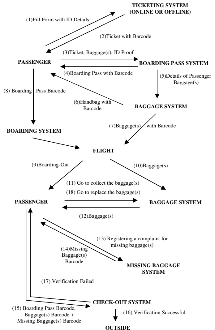
Figure 3: Our Proposed Approach
