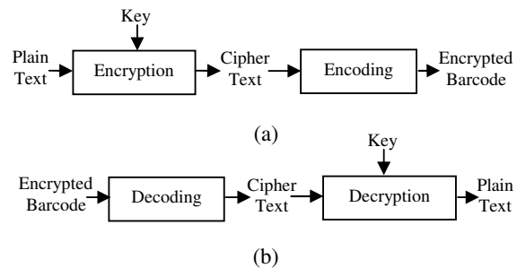
Figure 2: (a) Encryption and (b) Decryption in Barcode
