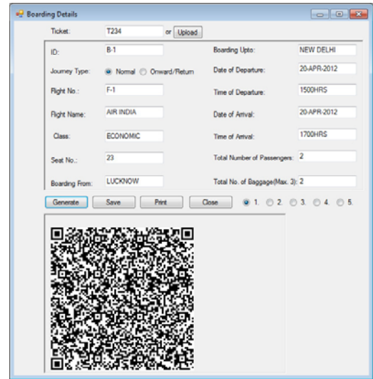
Figure 5: Boarding Pass Form
