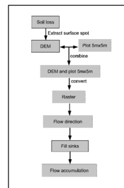
Fig 1 Soil flow direction flow chart.
