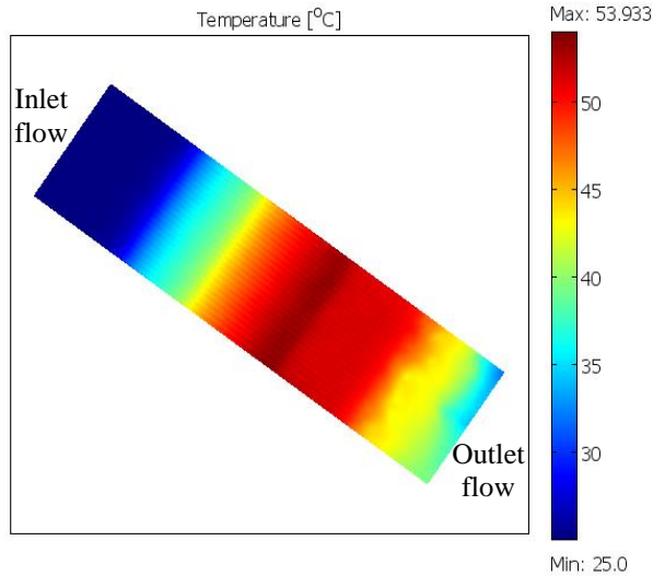
Fig. 3 2D Temperature distribution on the chip surface (half geometry model).
