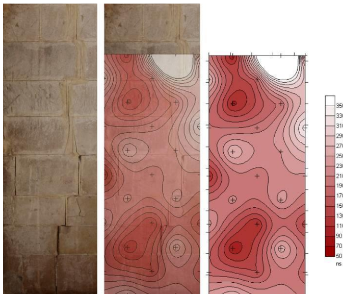
Figure 13. A lesion in the wall near the entrance central portal. Ultrasonic tomography processed with the measurements of pulse propagation time between the probes.
